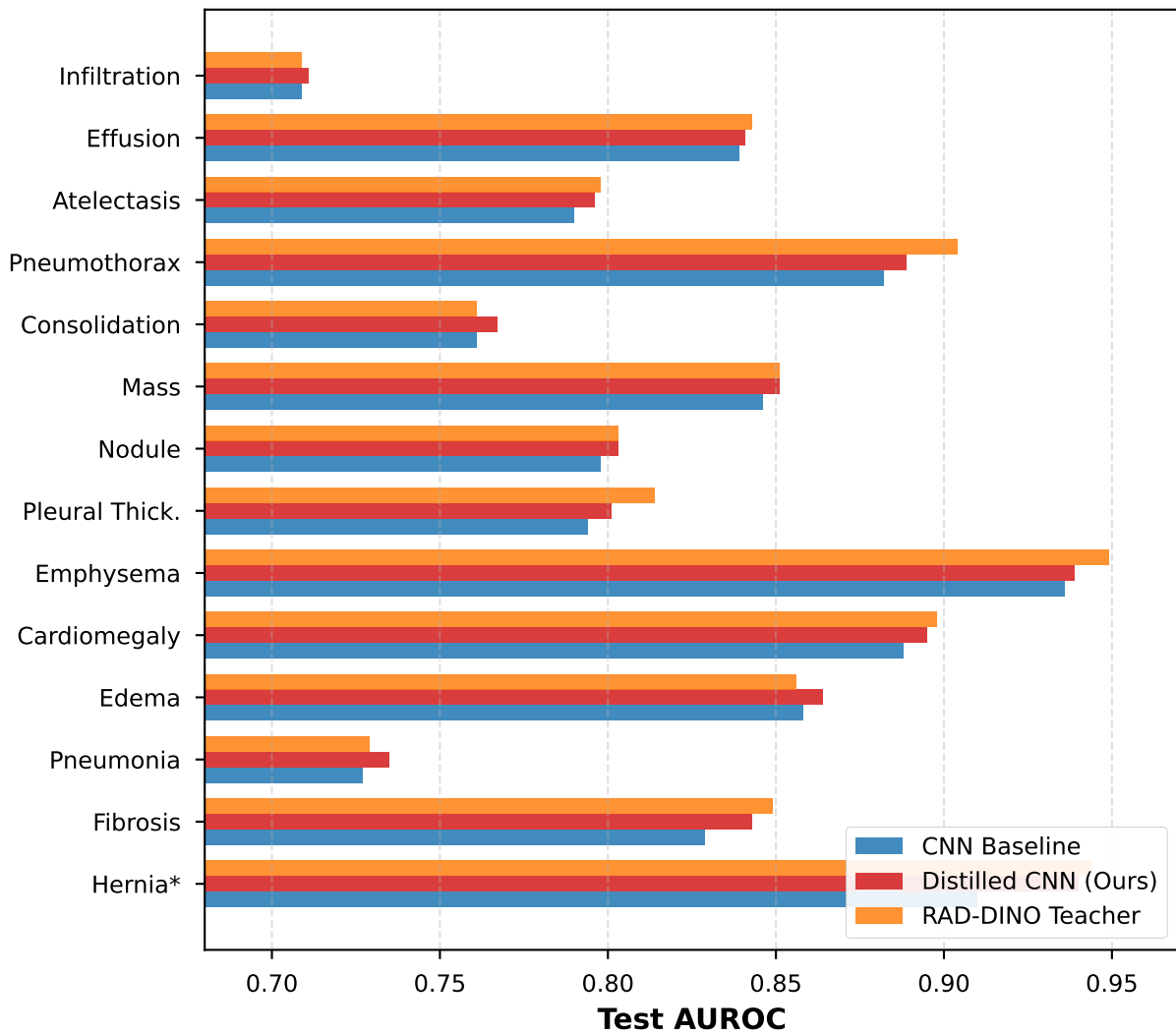
Per-Finding AUROC Comparison
