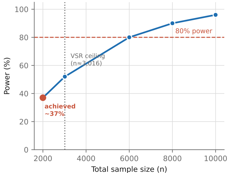
(b) Power assuming true effect = 0.267 log-odds
