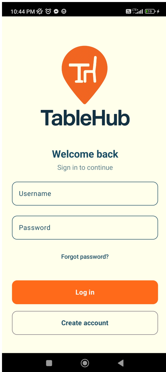
Figure 7: Login Screen
