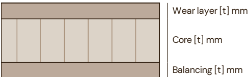
Section device at the product's true proportions; labels in millimetres frc
