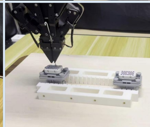
Wire Insertion
