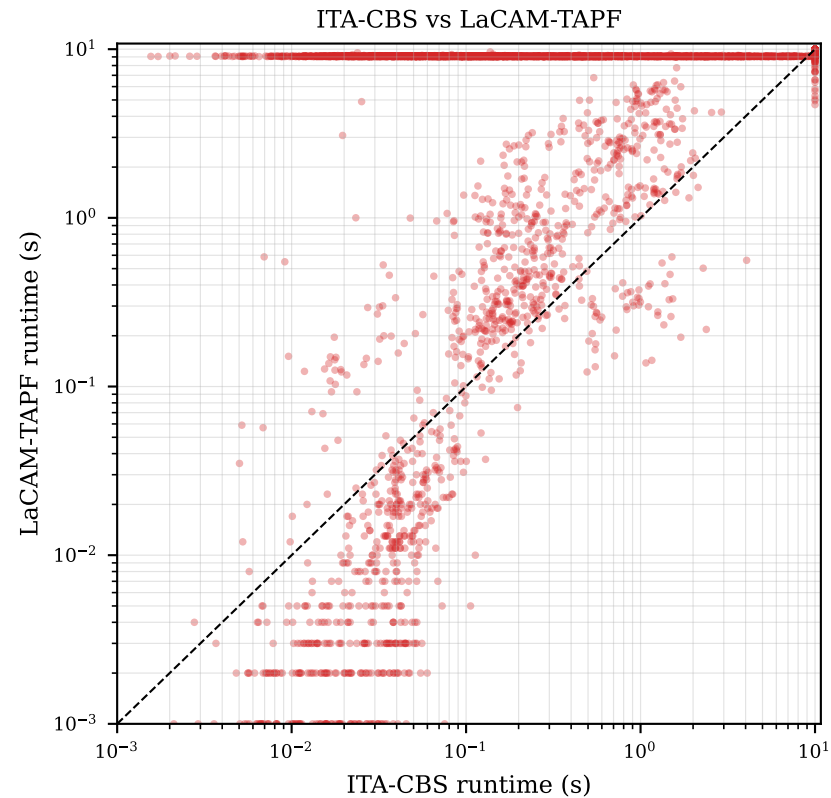
Figure 3 style: runtime scatter, timeouts capped at 10s
