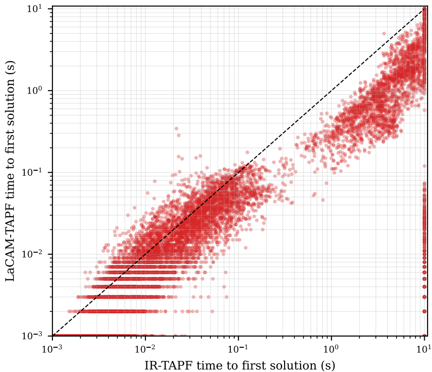
Figure 3b style: first-solution scatter, failures capped at 10s
