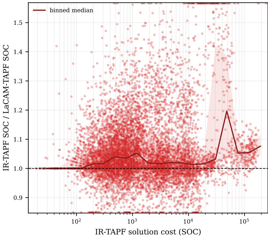
Figure 3c style: solution quality ratio
