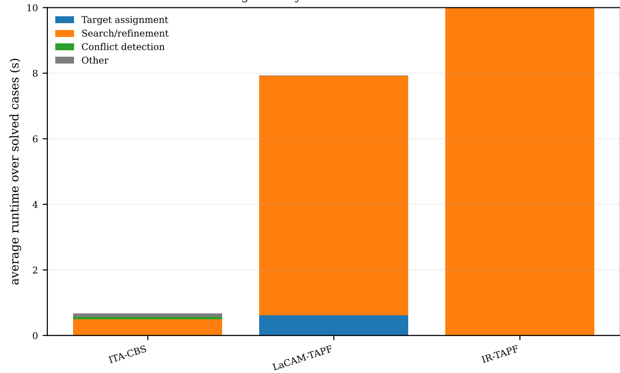
Figure 5 style: runtime breakdown
