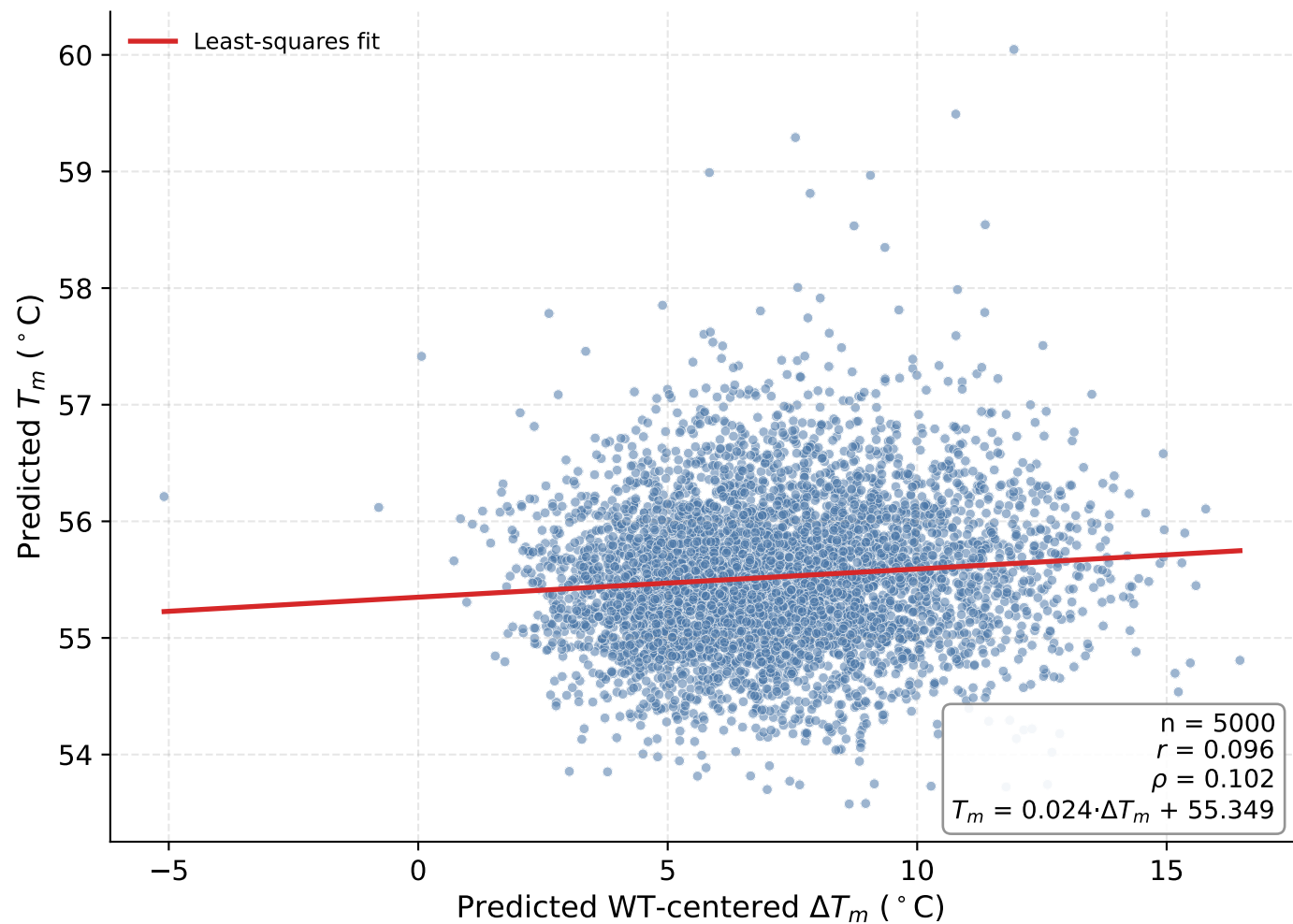
Predicted \Delta T_m vs Predicted T_m
