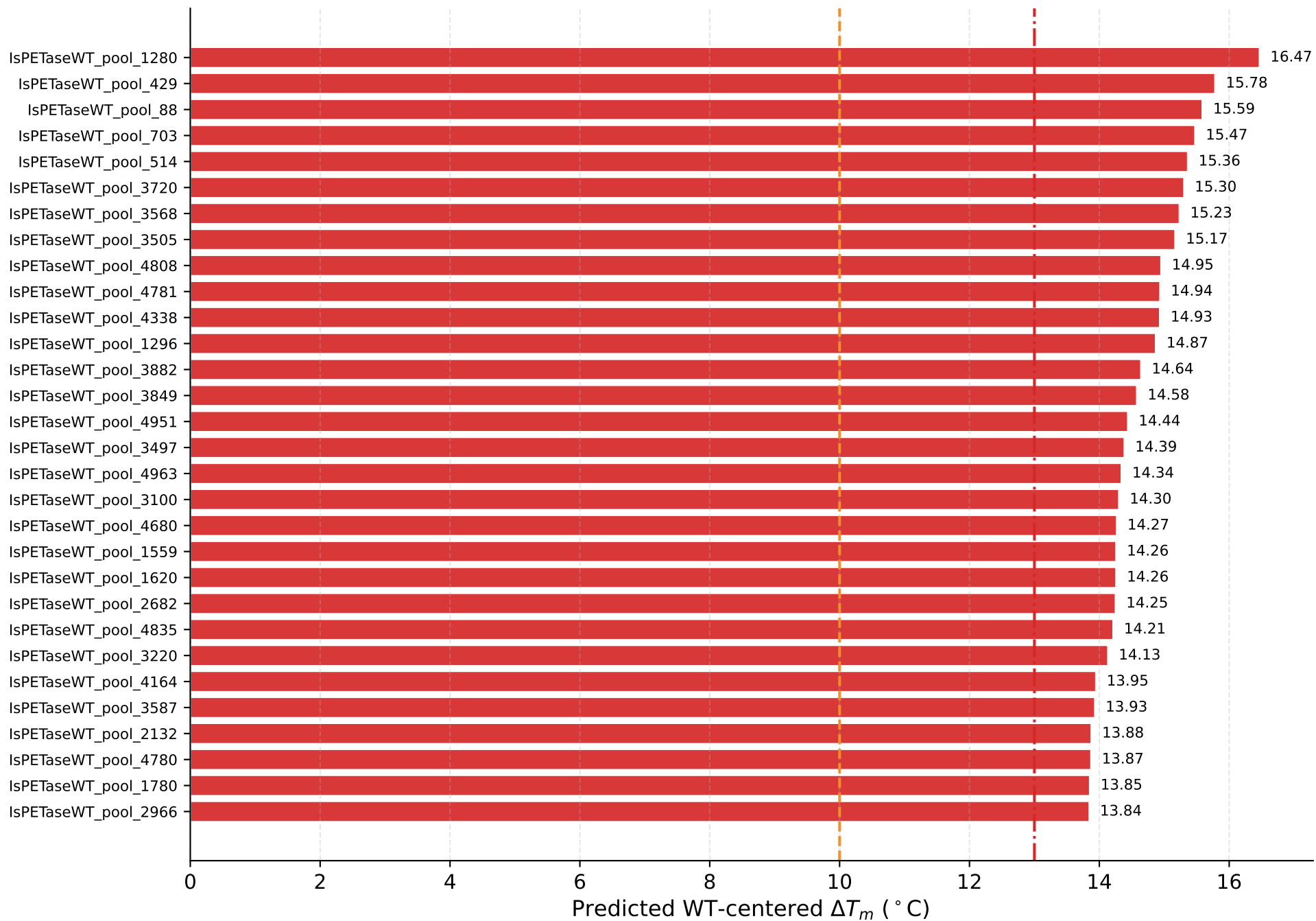
Top 30 Candidates by Predicted WT-Centered \Delta T_m
