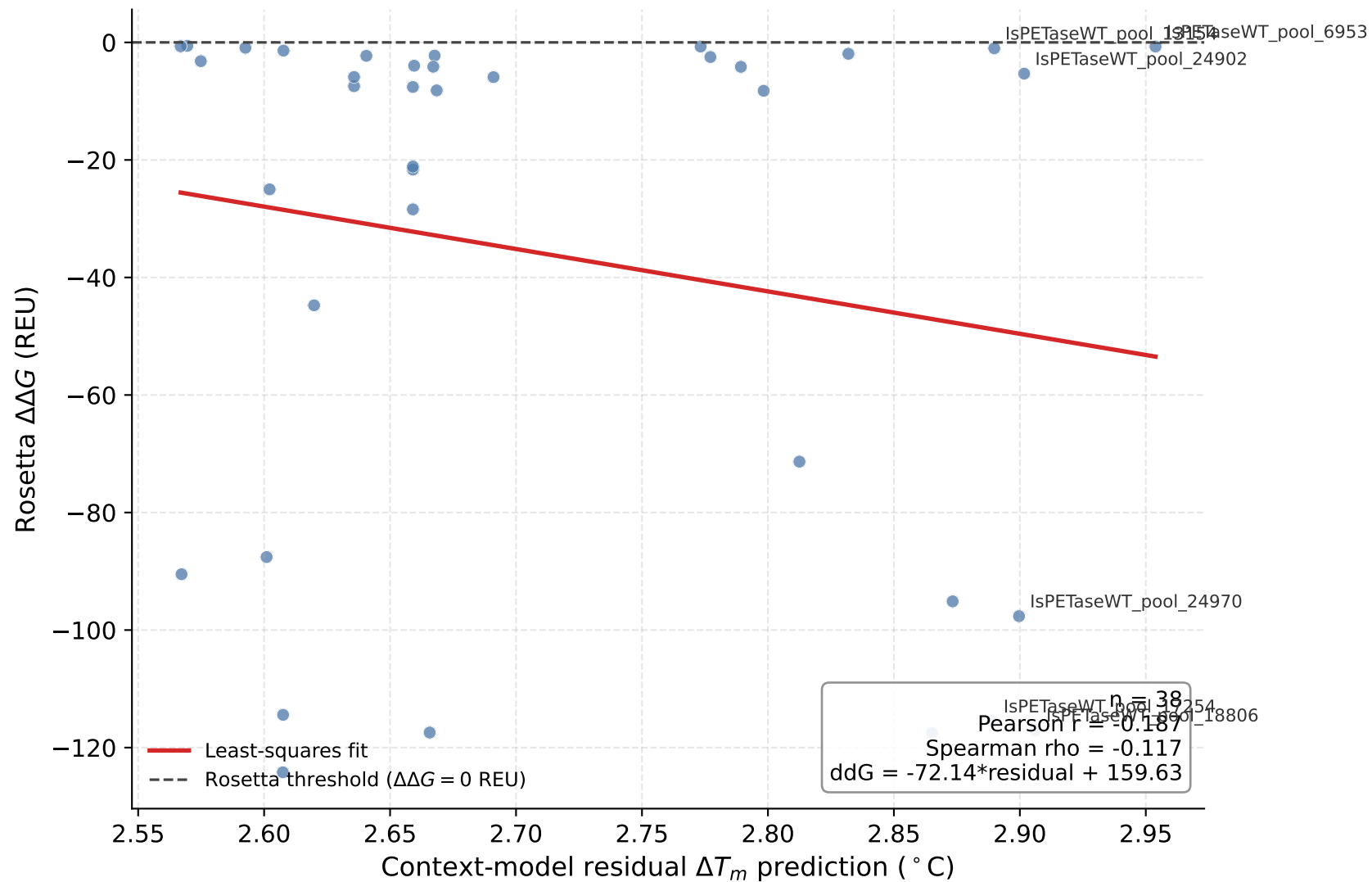
Context Residual vs Rosetta \Delta\Delta G for Final Shortlist
