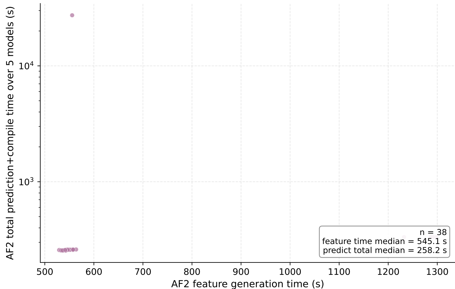
AlphaFold Runtime Profile Per Final Candidate
