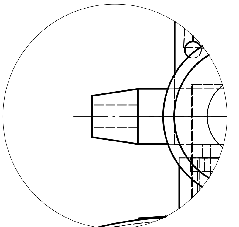
DETALLE E (2:1) Tobera
