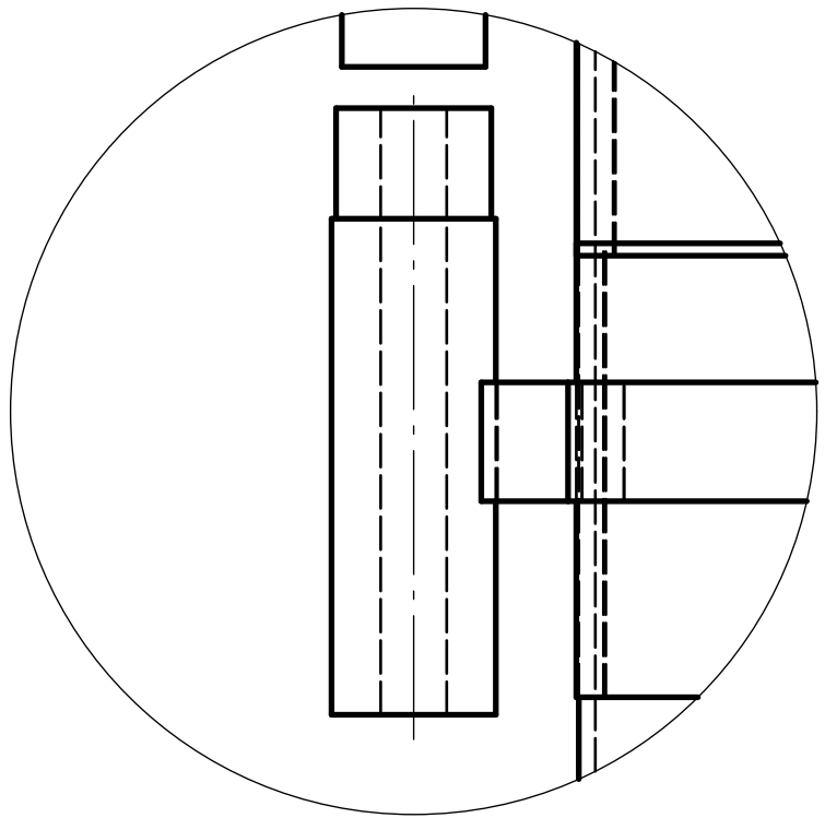
DETALLE E (1:1) Tobera y portatobera
