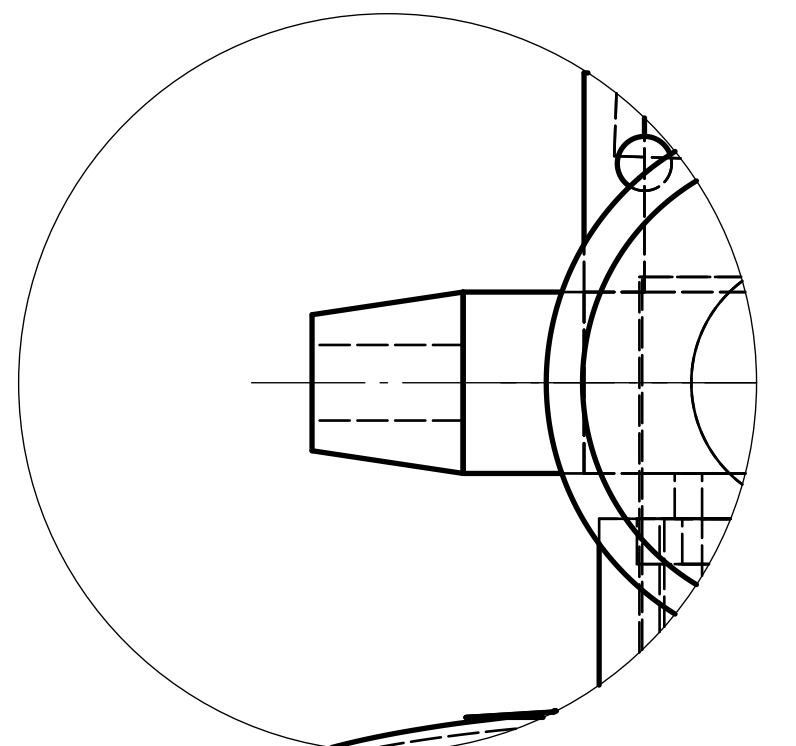
DETALLE E (2:1) Tobera
