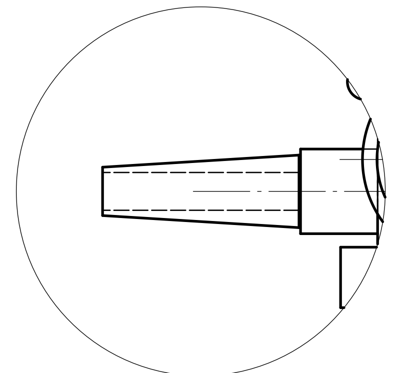
DETALLE E (2:1) Tobera
