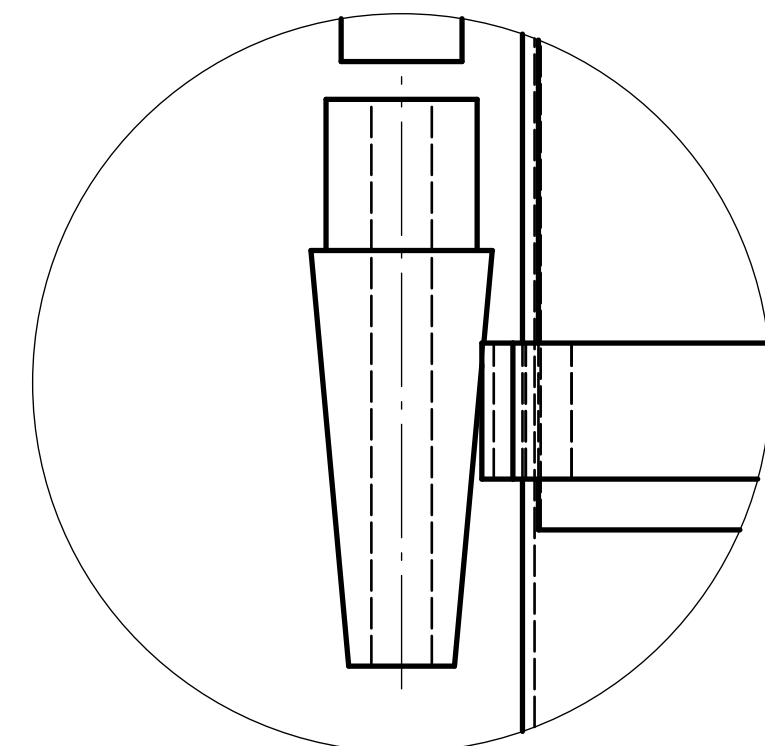
DETALLE E (1:1) Tobera y portatobera
