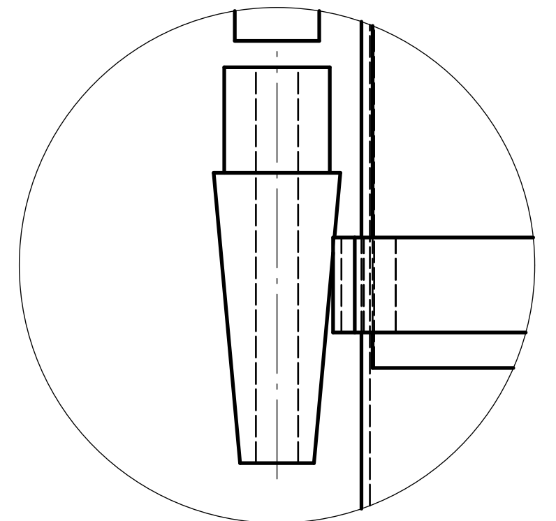
DETALLE E (1:1) Tobera y portatobera
