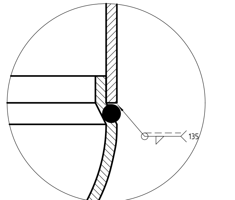
DETALLE D (1:1)
