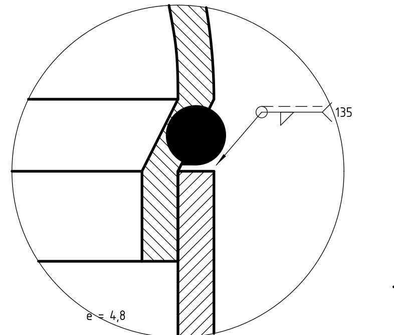
DETALLE C (2:1)
