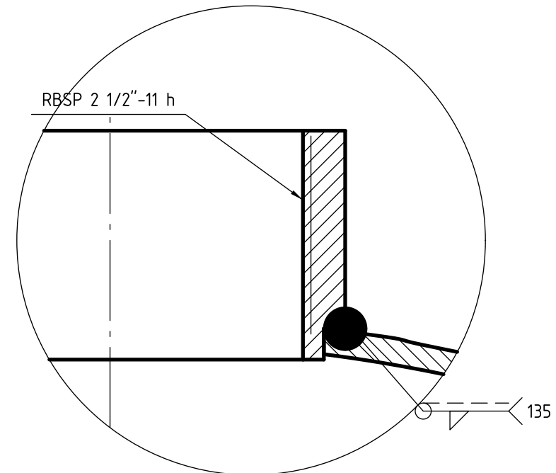
DETALLE B (1:1)
