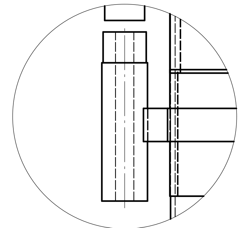
DETALLE E (1:1) Tobera y portatobera
