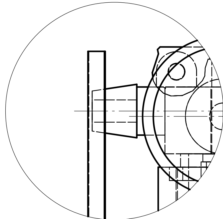
DETALLE E (2:1) Tobera
