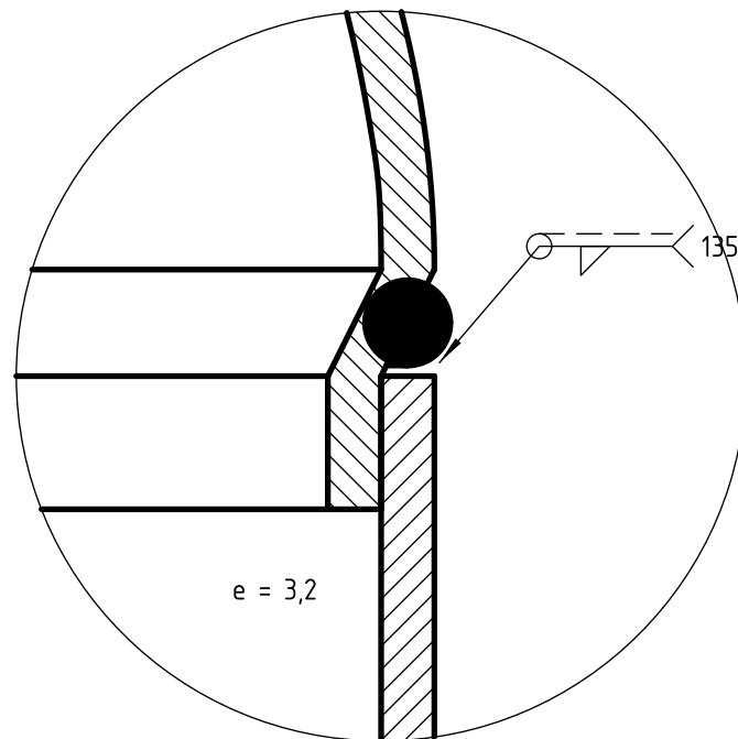
DETALLE C (2:1)
