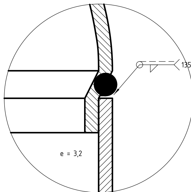
DETALLE C (2:1)
