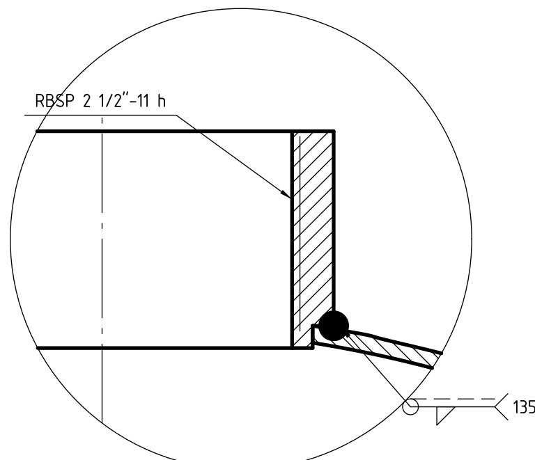
DETALLE B (1:1)
