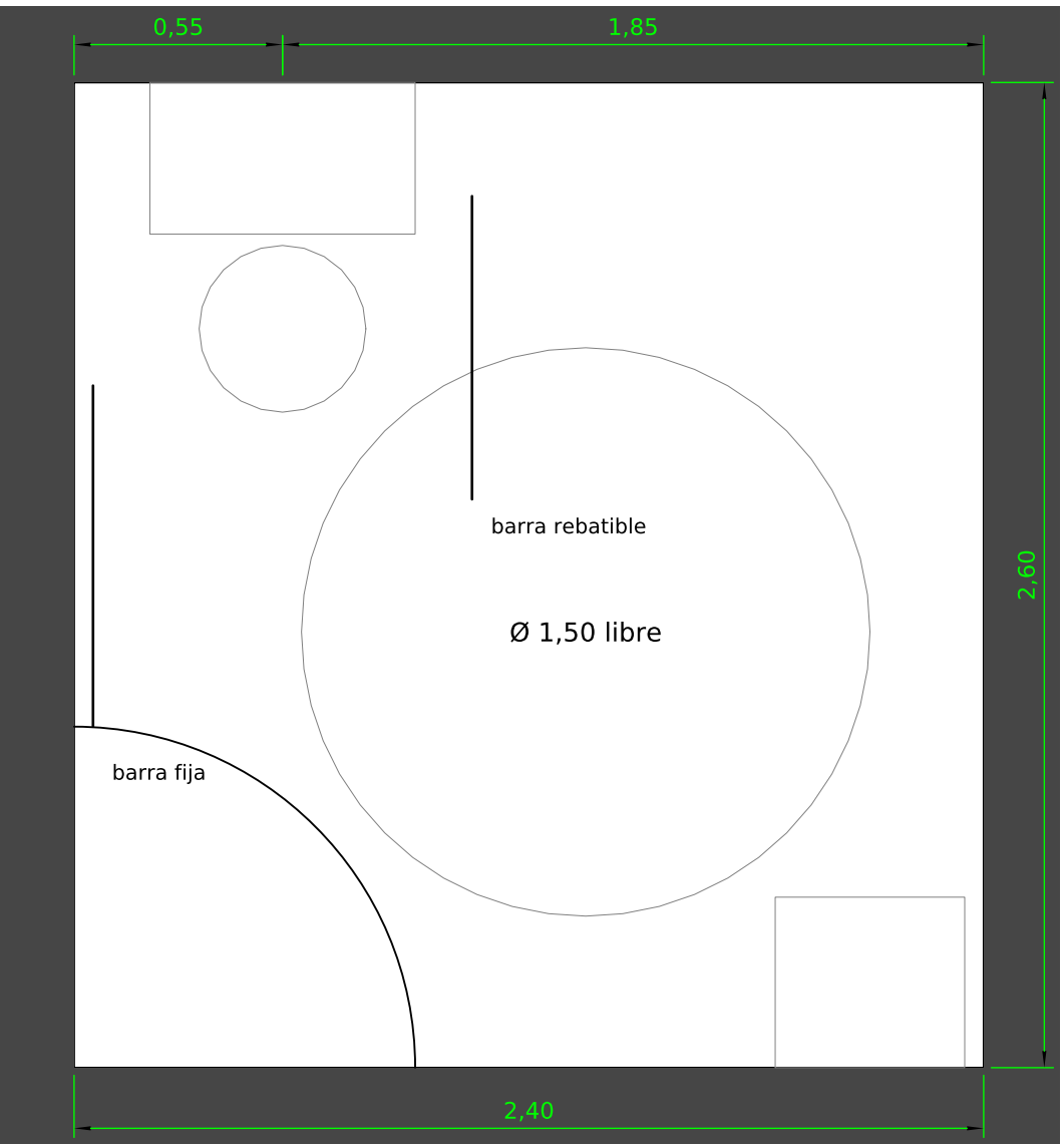
SANITARIO ACCESIBLE - 1:20 (Ley 24.314, Dec. 914/97)
