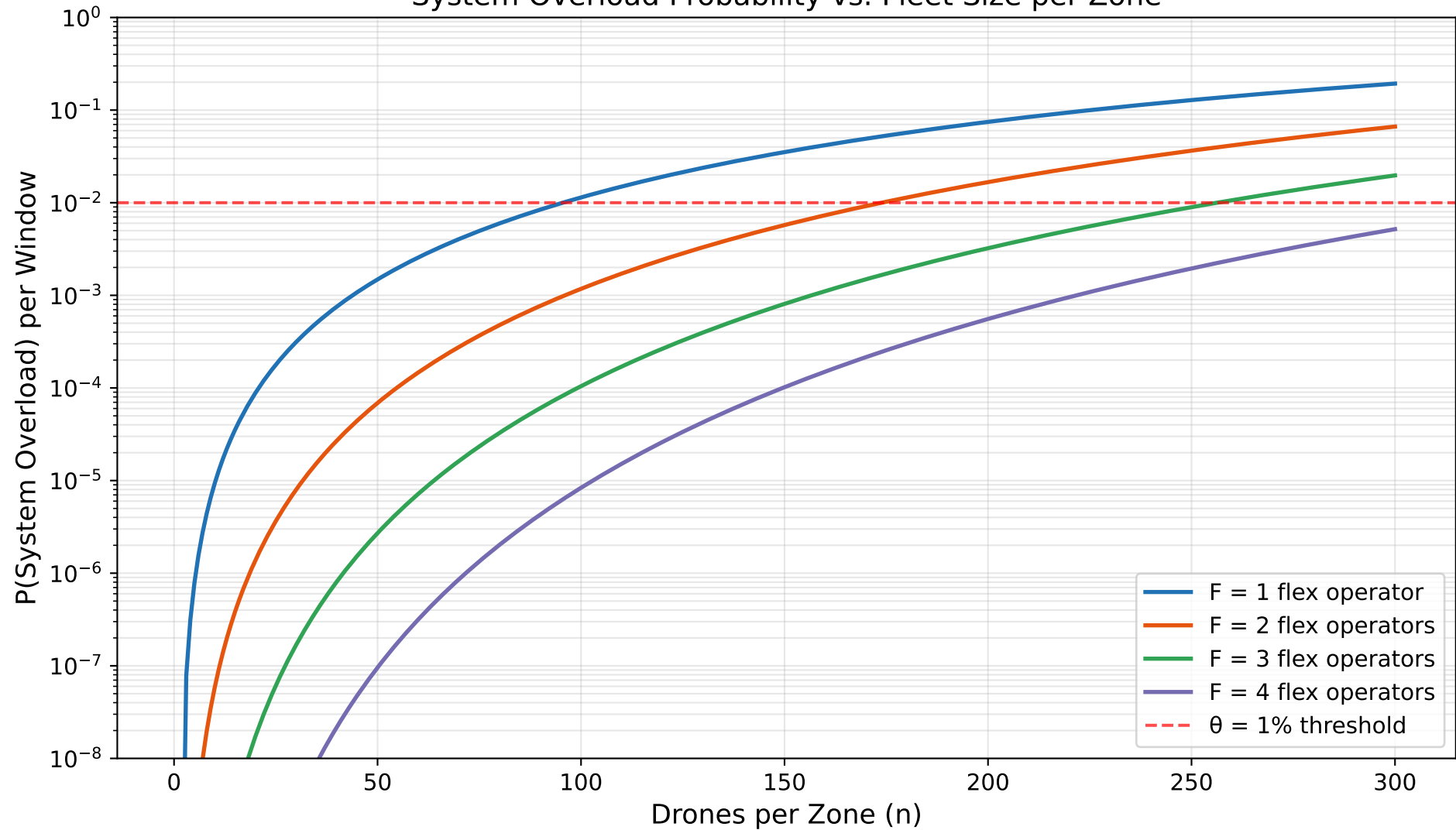
System Overload Probability vs. Fleet Size per Zone
