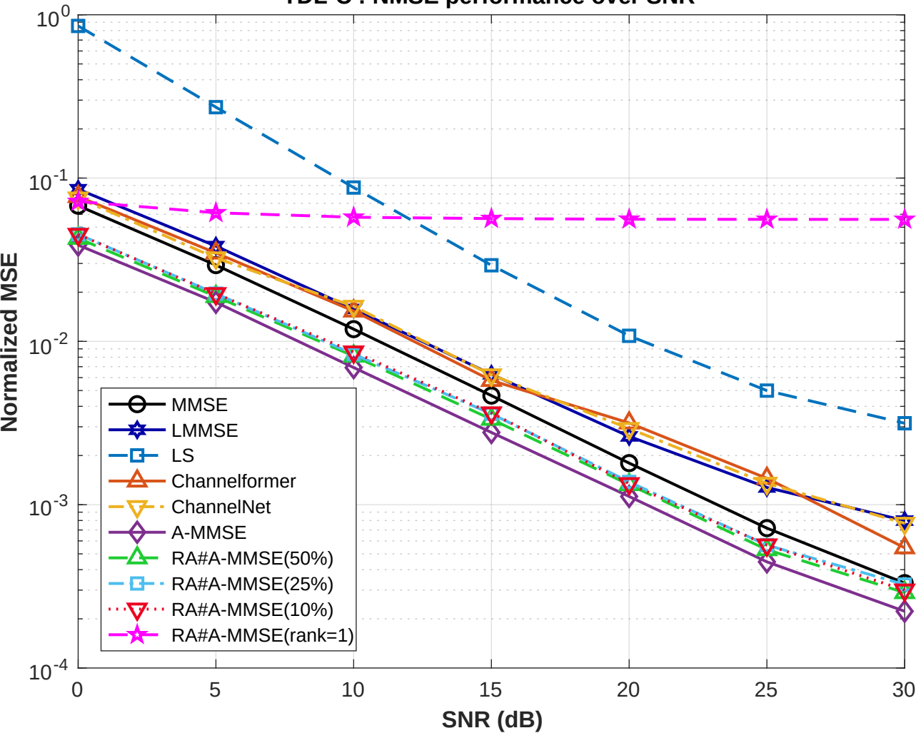
TDL-C : NMSE performance over SNR
