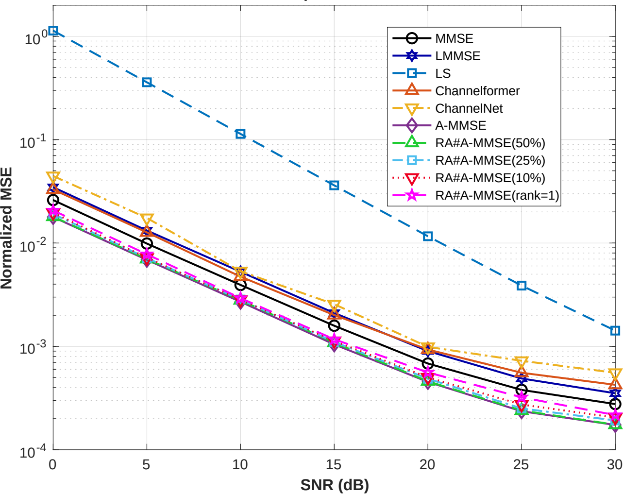
TDL-A : NMSE performance over SNR
