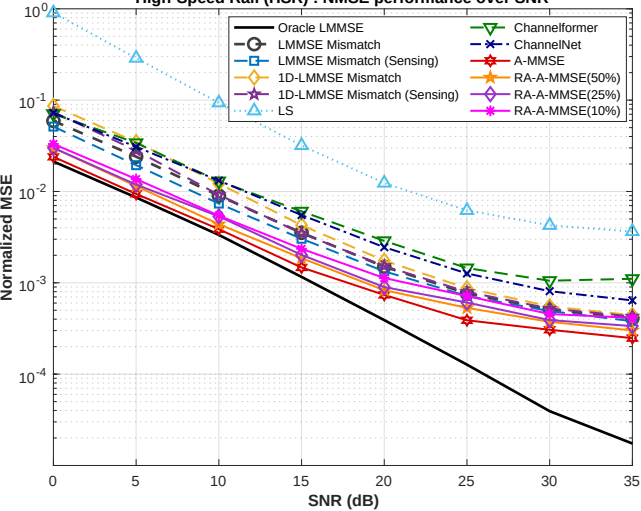
High-Speed Rail (HSR) : NMSE performance over SNR
