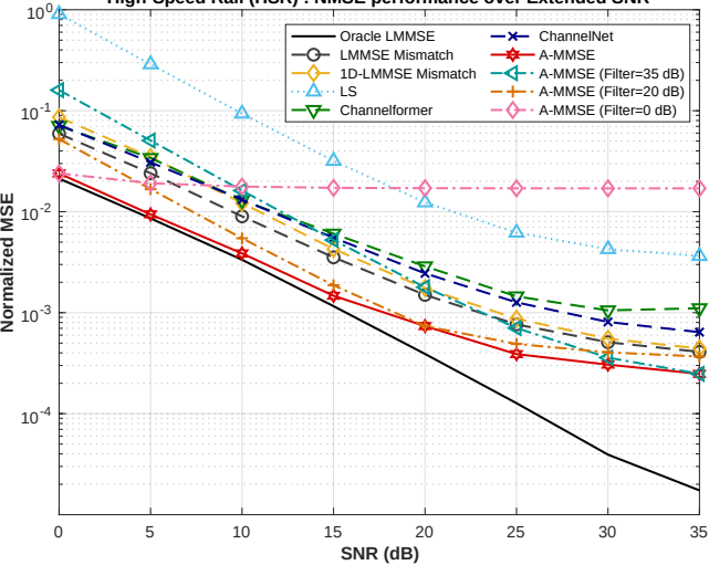
High-Speed Rail (HSR) : NMSE performance over Extended SNR
