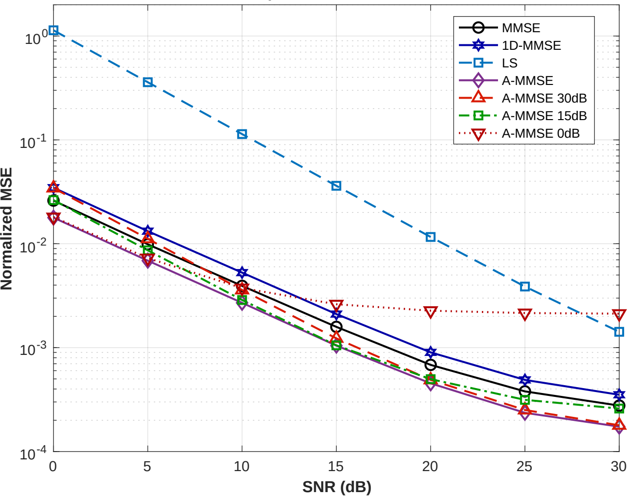
TDL-A : NMSE performance over Extended SNR
