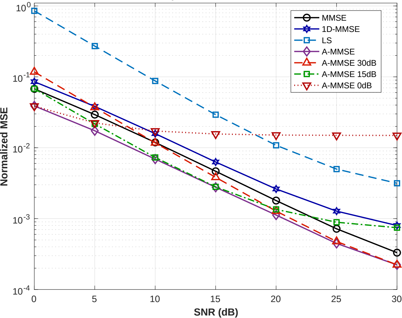
TDL-C : NMSE performance over Extended SNR
