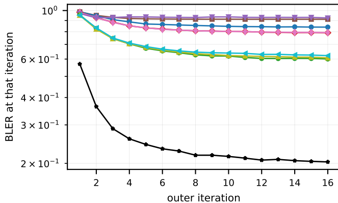
(c) BLER per iteration
