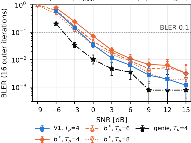
(a) BLER, V1 with 4 pilots vs GMM with 4/6/8 8 \times 4 , T=16 , N_{\text{train}} = 1.6 \times 10^5 (equal budget)
