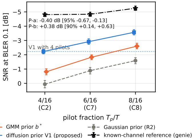
(b) SNR at BLER 0.1 vs pilot overhead (up = better; 90% unpaired intervals)
