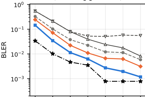
(d) SV8e: clustered Saleh-Valenzuela (UNGATED)
