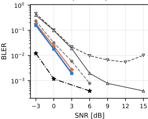
(d) SV8e: clustered Saleh-Valenzuela (UNGATED)
