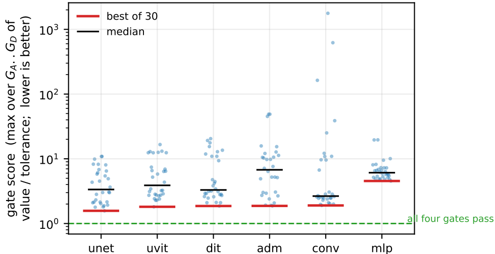
Architecture at equal budget: 30 random trials each
