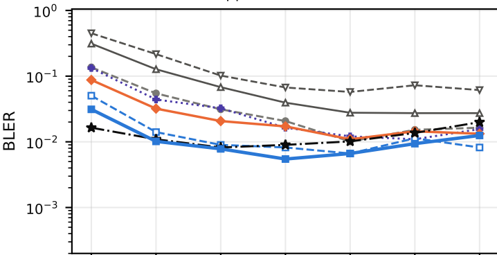
(c) Rx rotation 15^\circ , 16 \times 4
