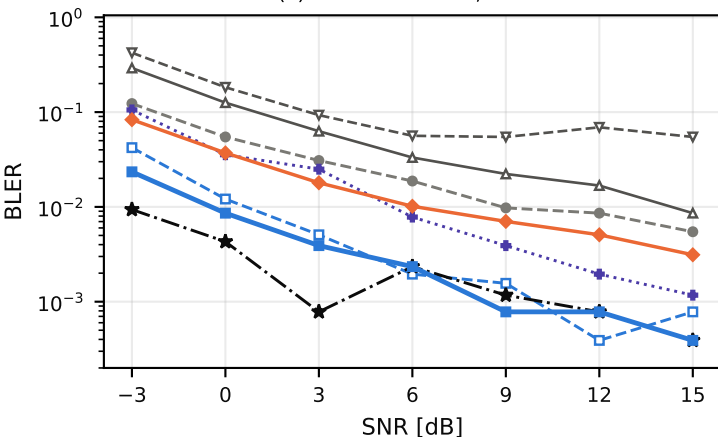
(c) Rx rotation 15^\circ , 16 \times 4
