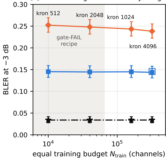
(b) the advantage holds at every budget
