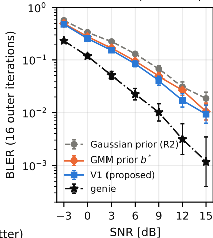
(b) BLER on 3GPP 38.901 UMi 28 GHz (UNGATED)
