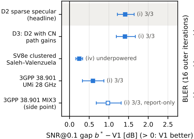
(a) V1 vs equal-budget GMM b^* , per channel model (90% paired CI)
