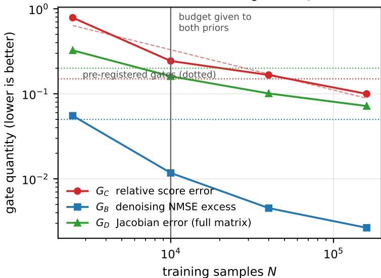
Learned score vs the frozen gates: G_C \propto N^{-0.47}
