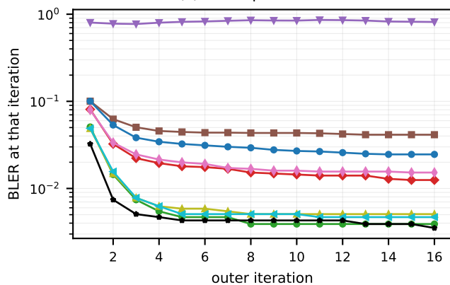
(c) BLER per iteration
