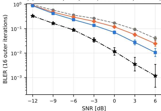
(d) UMi28 C9 (32×4): BLER, 95% Wilson (UNGATED)
