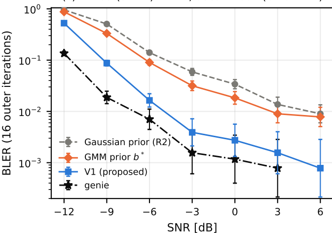
(c) D2 C9 (32×4): BLER, 95% Wilson (UNGATED)
