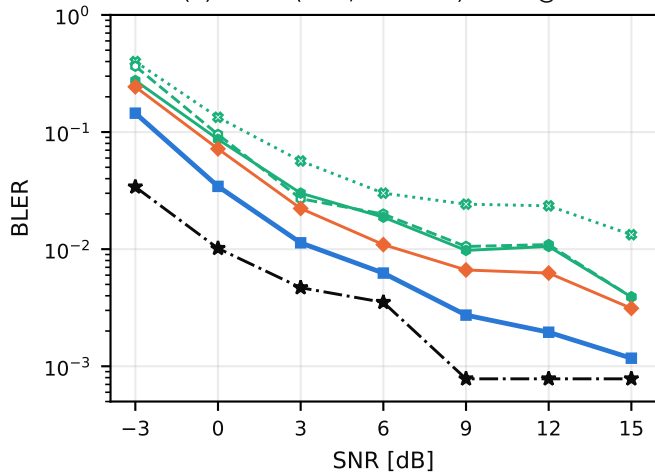
(b) D2 C2 (8×4, headline): BLER@16
