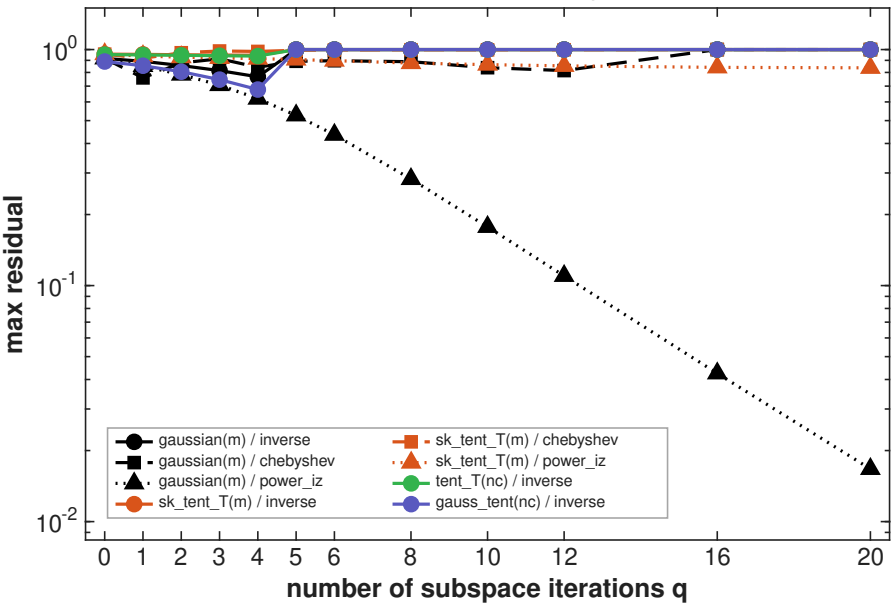
max residual ( Z = \text{Tsym}^{-1} )
