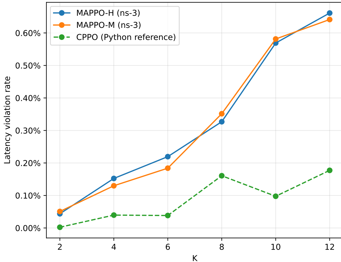
Latency
