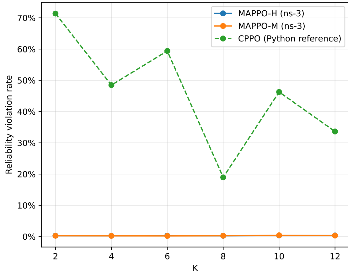
Reliability
