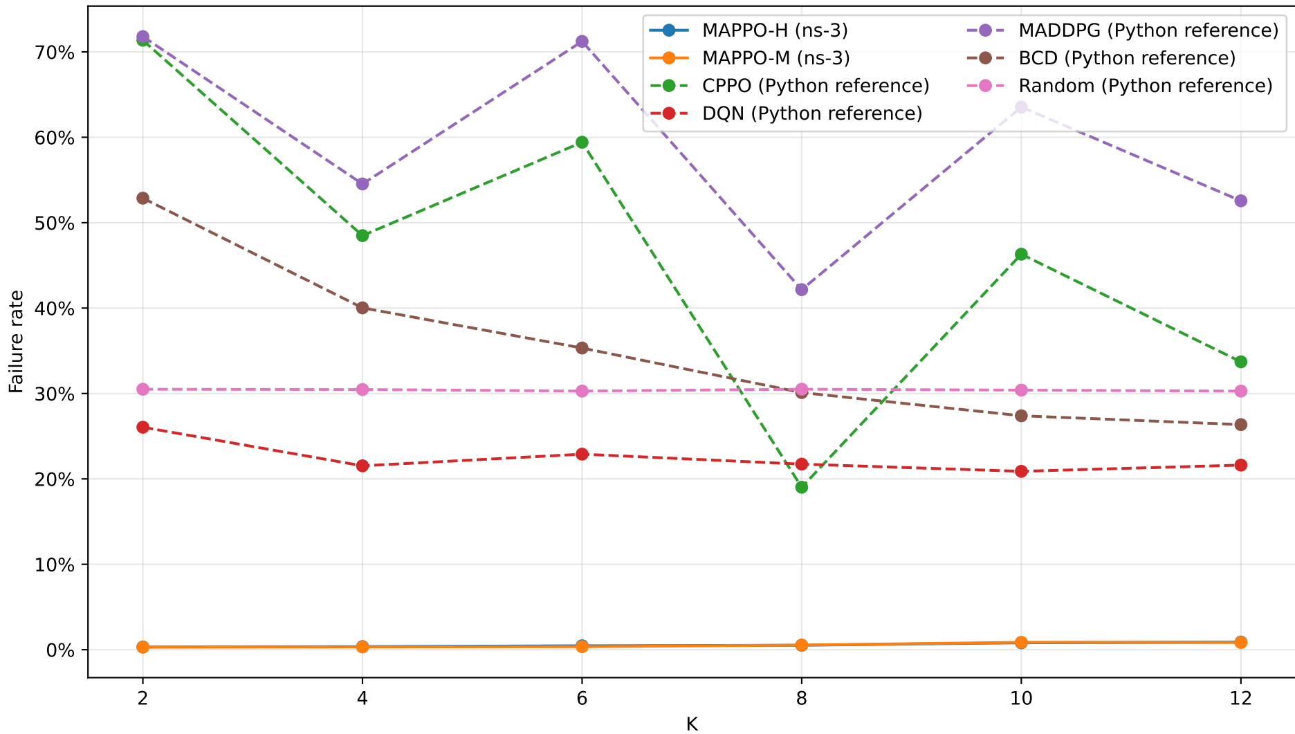
Figure 8: Failure rate vs K
