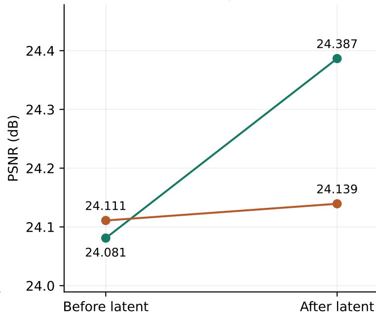
Placement interacts with the fusion operator Full-image test
