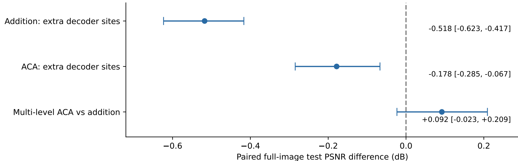
Final layout comparisons: mean differences and recorded 95% intervals Intervals describe image sampling, not training-seed variability
