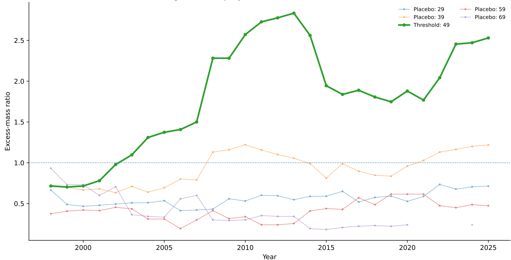
Bunching at 49 Employees Relative to Placebo Thresholds
