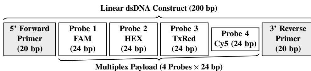
Figure 2.2. Molecular layout of the 200 bp DNA taggant construct.
